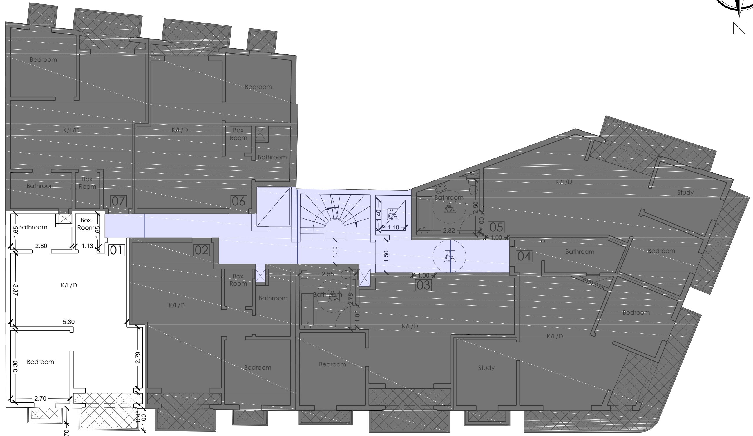
Second Floor
